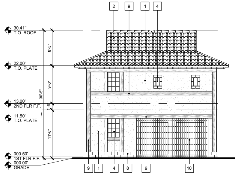
RECTORY SOUTH ELEVATION
