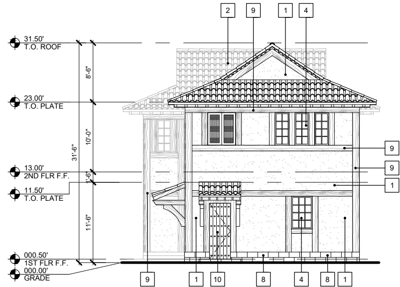
RECTORY NORTH ELEVATION
